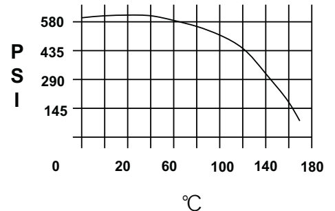
PRESS. VS. TEMP. CURVE
