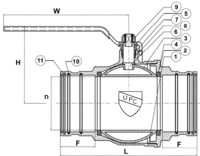
XLC 2 1/2" TO 4"
