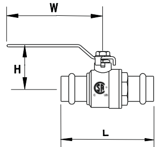
1/2" TO 2" STANDARD
